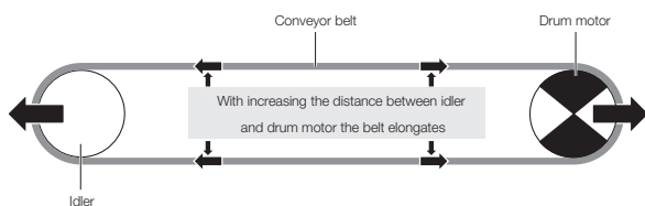
Fig.: Belt elongation
