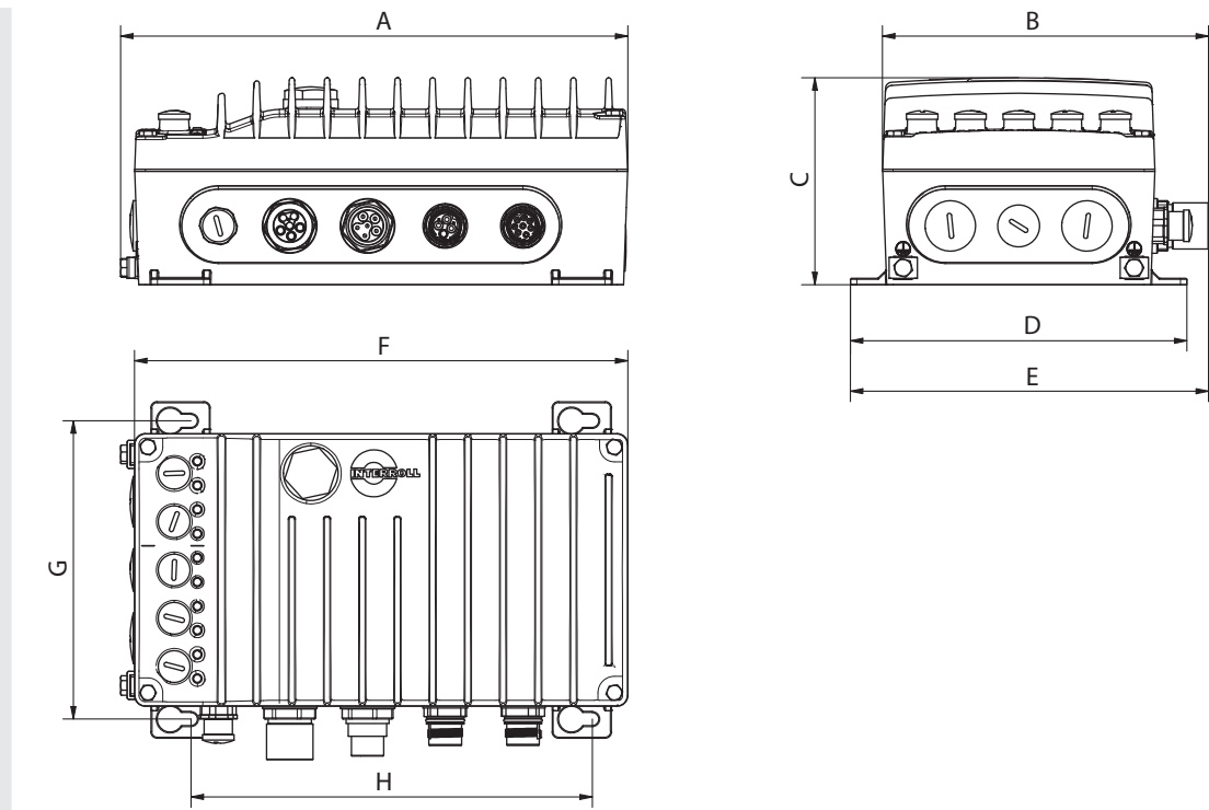
Fig.: FC 1000, wall-mounted, size 1 & 2
