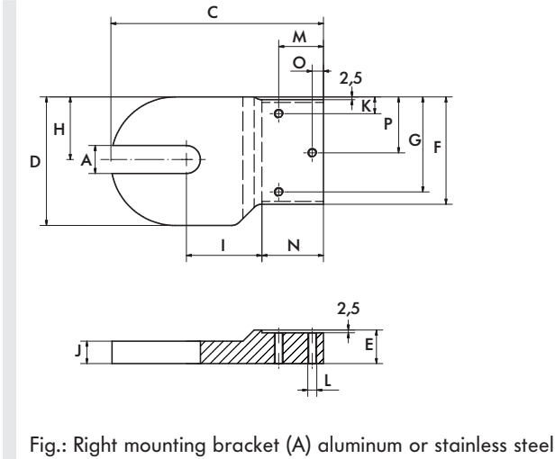
Fig.: Right mounting bracket (A) aluminum or stainless steel
