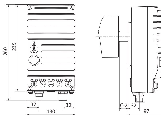
Fig.: FC1000, motor-mounted, size 2
