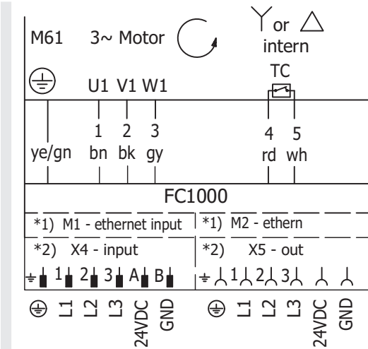
Fig.: 3-phase, 4-core cable, winding for 1 voltage, delta or star connection
