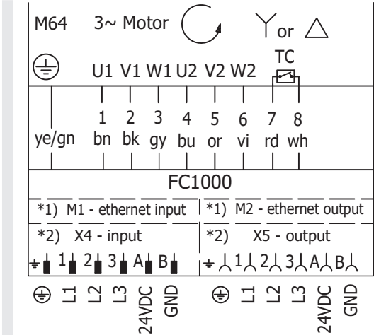
FC 1000 3-phase asynchronous motor
