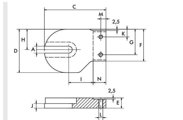
Fig.: Right mounting bracket (A) aluminum or stainless steel
