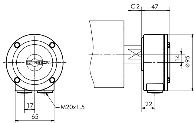
Fig.: Terminal box, aluminum
