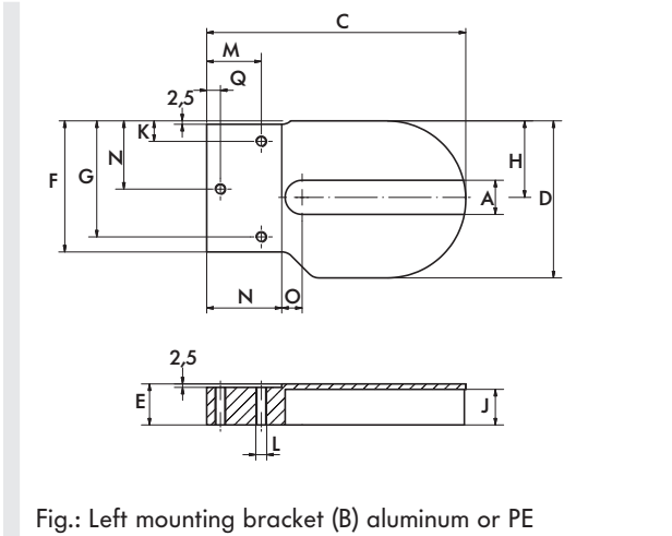
Fig.: Left mounting bracket (B) aluminum or PE
